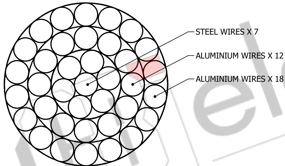
SECTIONAL VIEW
