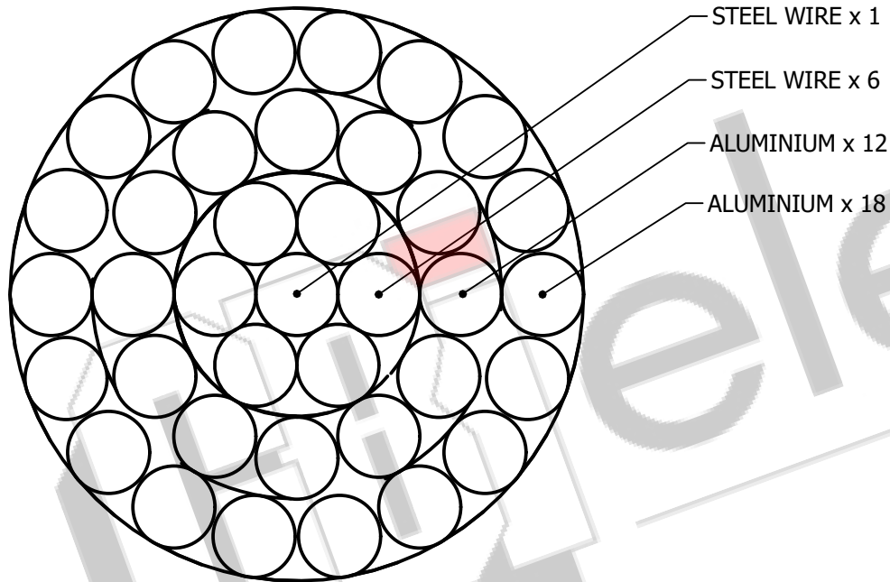
SECTIONAL VIEW
