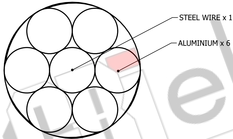
SECTIONAL VIEW
