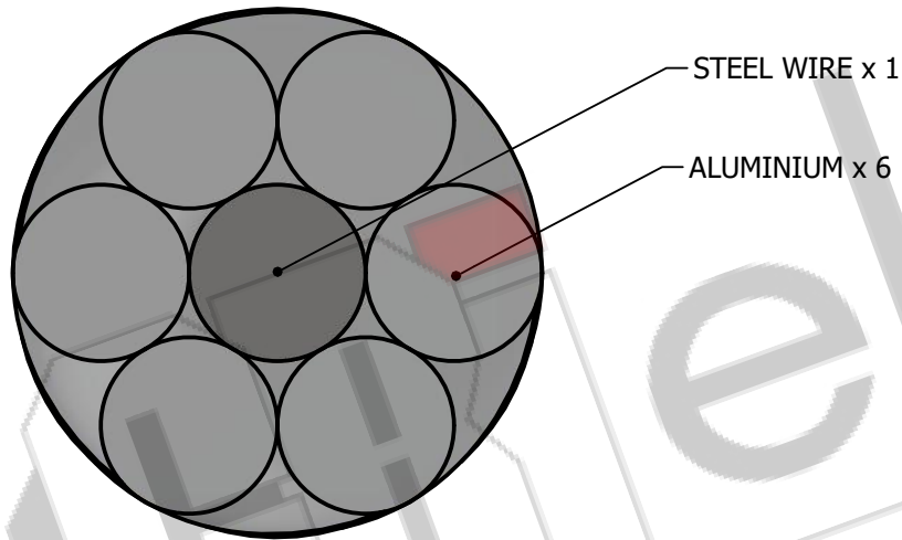
SECTIONAL VIEW
