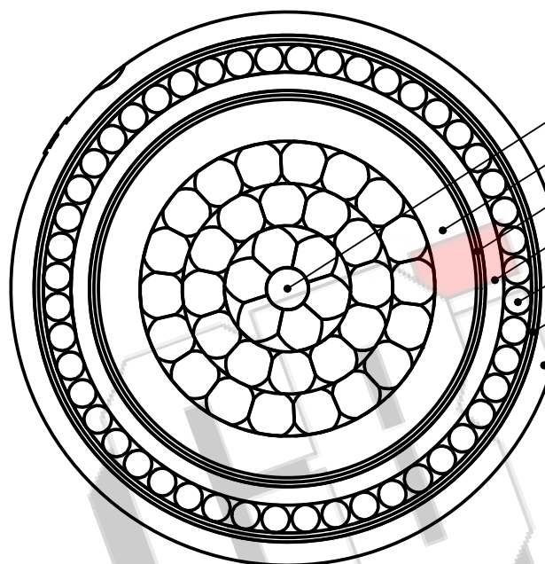
SECTIONAL VIEW
