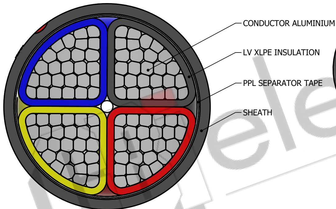
SECTIONAL VIEW
