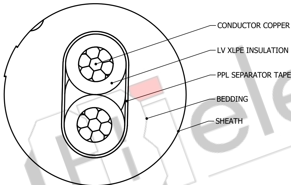
SECTIONAL VIEW
