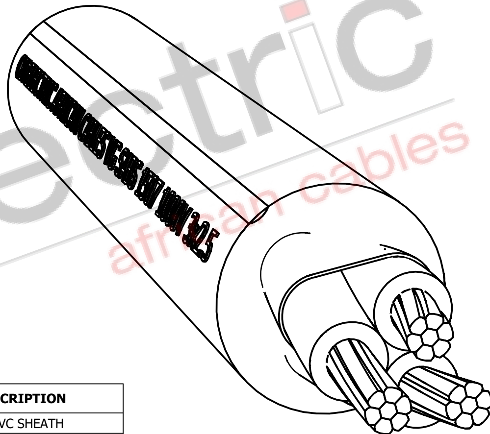
ISOMETRIC VIEW
