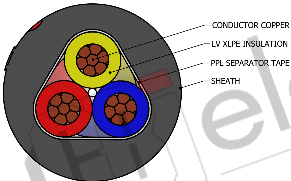
SECTIONAL VIEW
