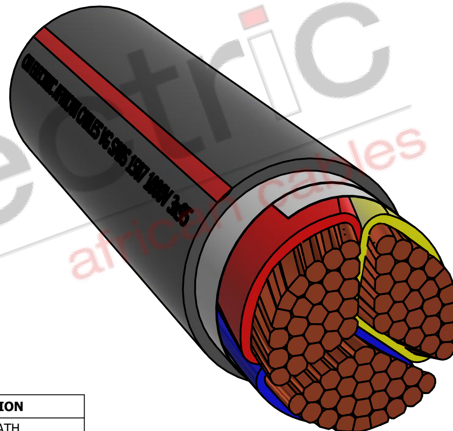
ISOMETRIC VIEW
