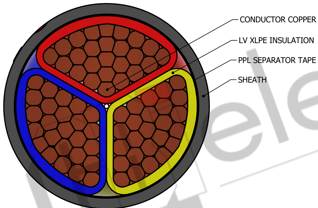
SECTIONAL VIEW
