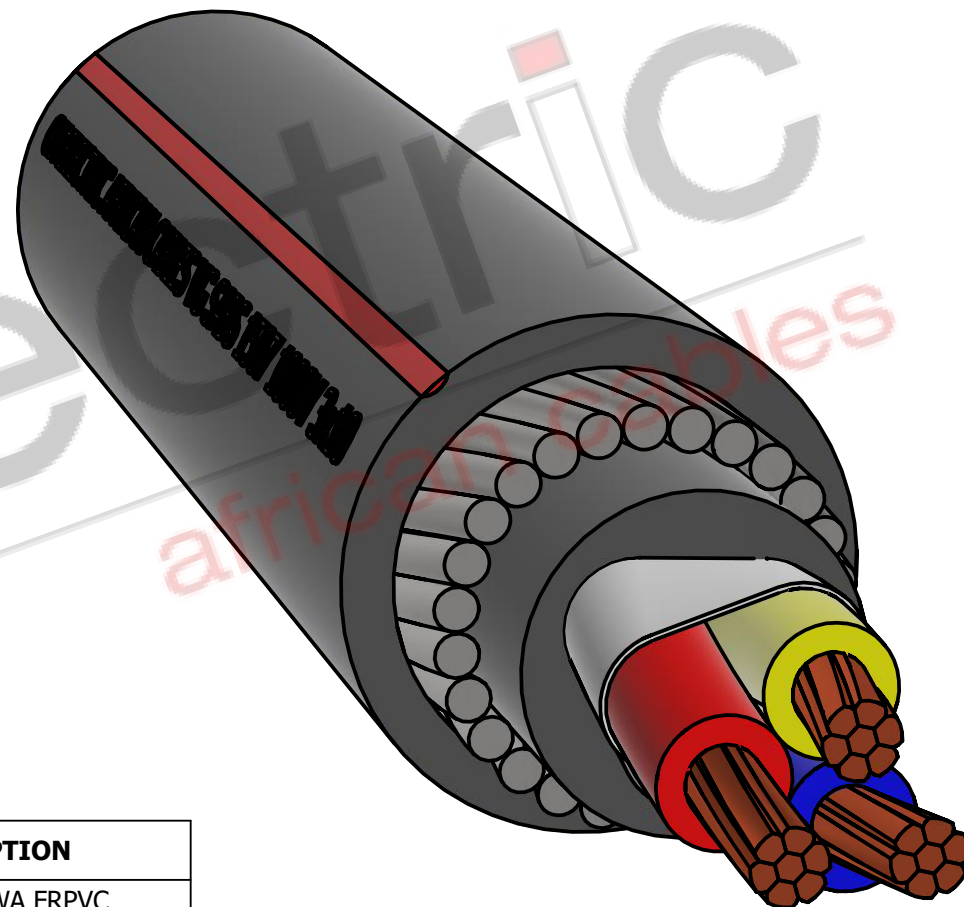
ISOMETRIC VIEW
