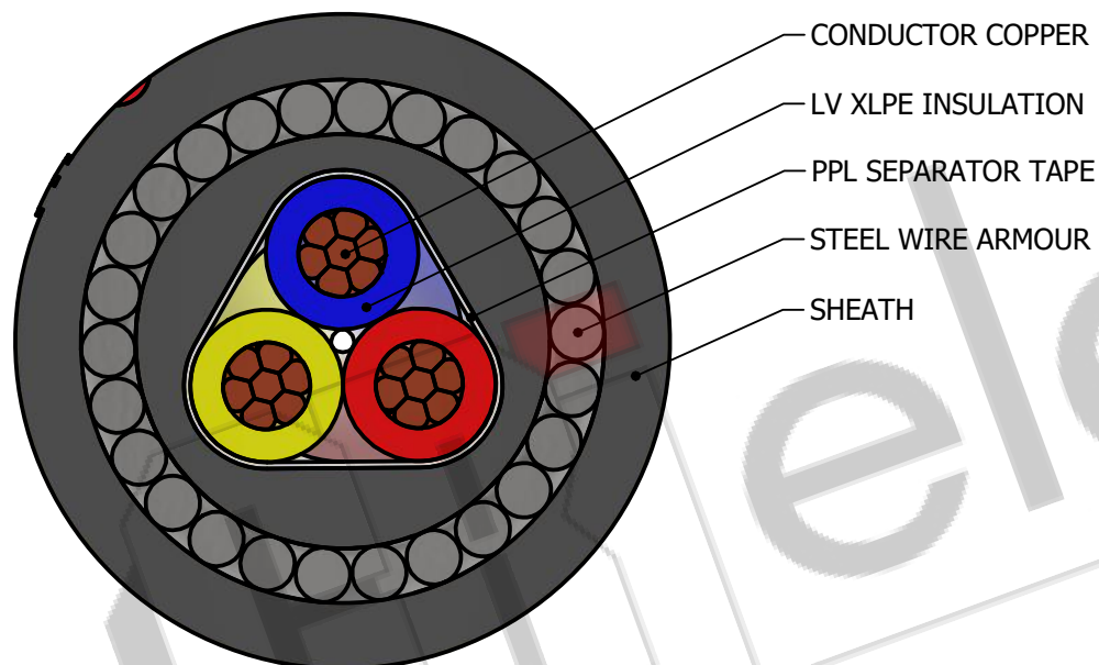
SECTIONAL VIEW
