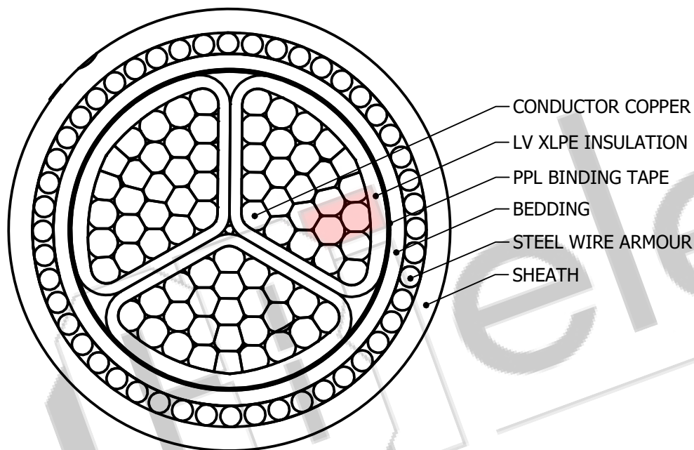
SECTIONAL VIEW
