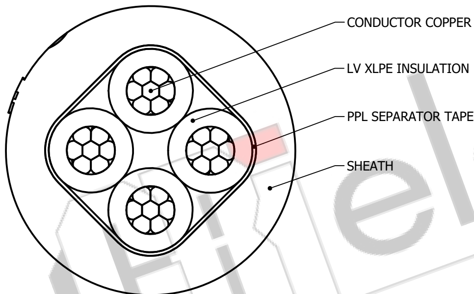
SECTIONAL VIEW
