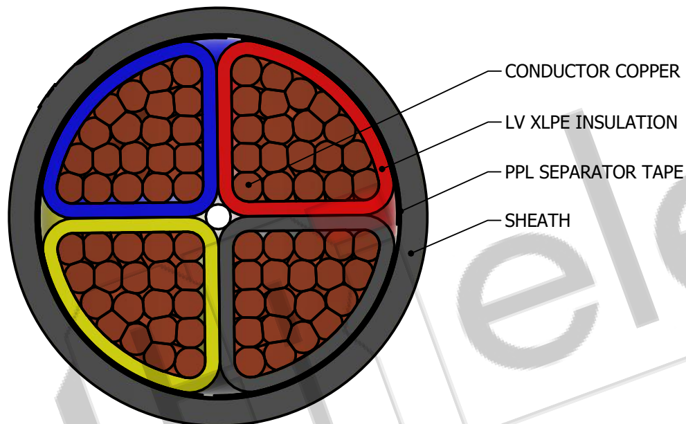
SECTIONAL VIEW
