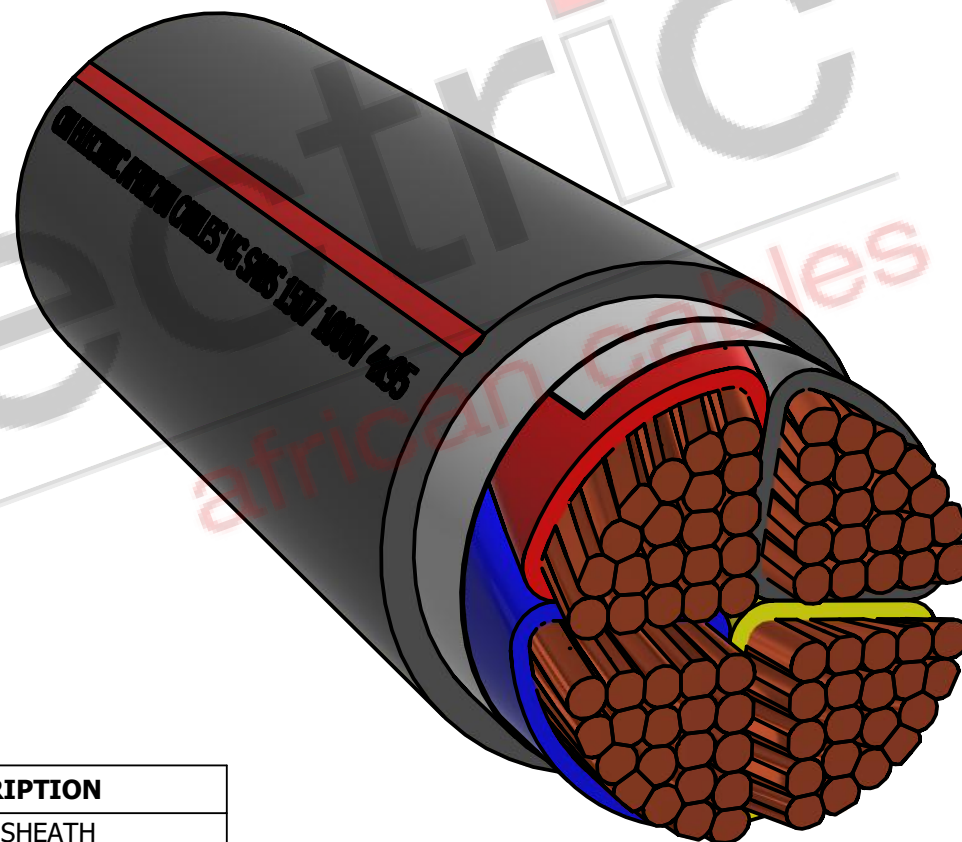
ISOMETRIC VIEW
