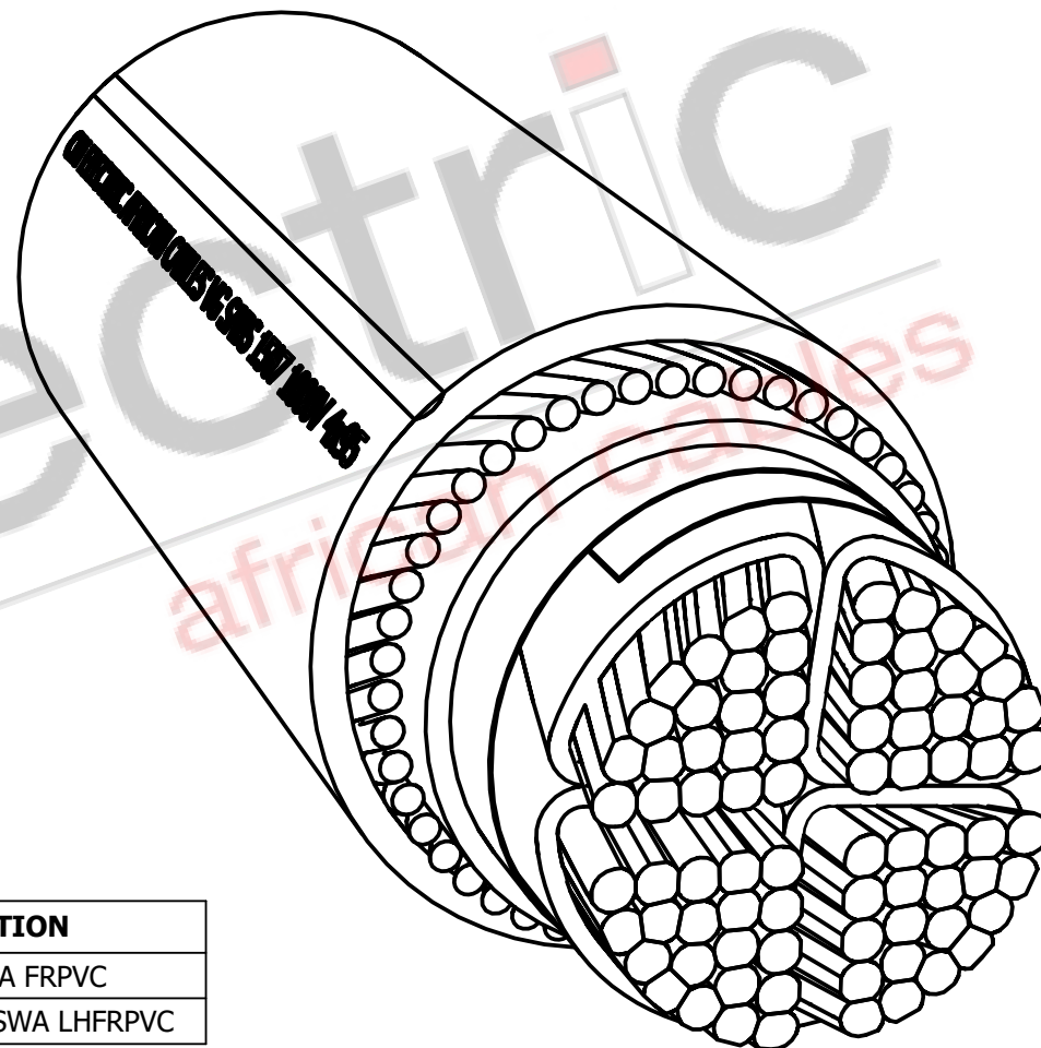
ISOMETRIC VIEW
