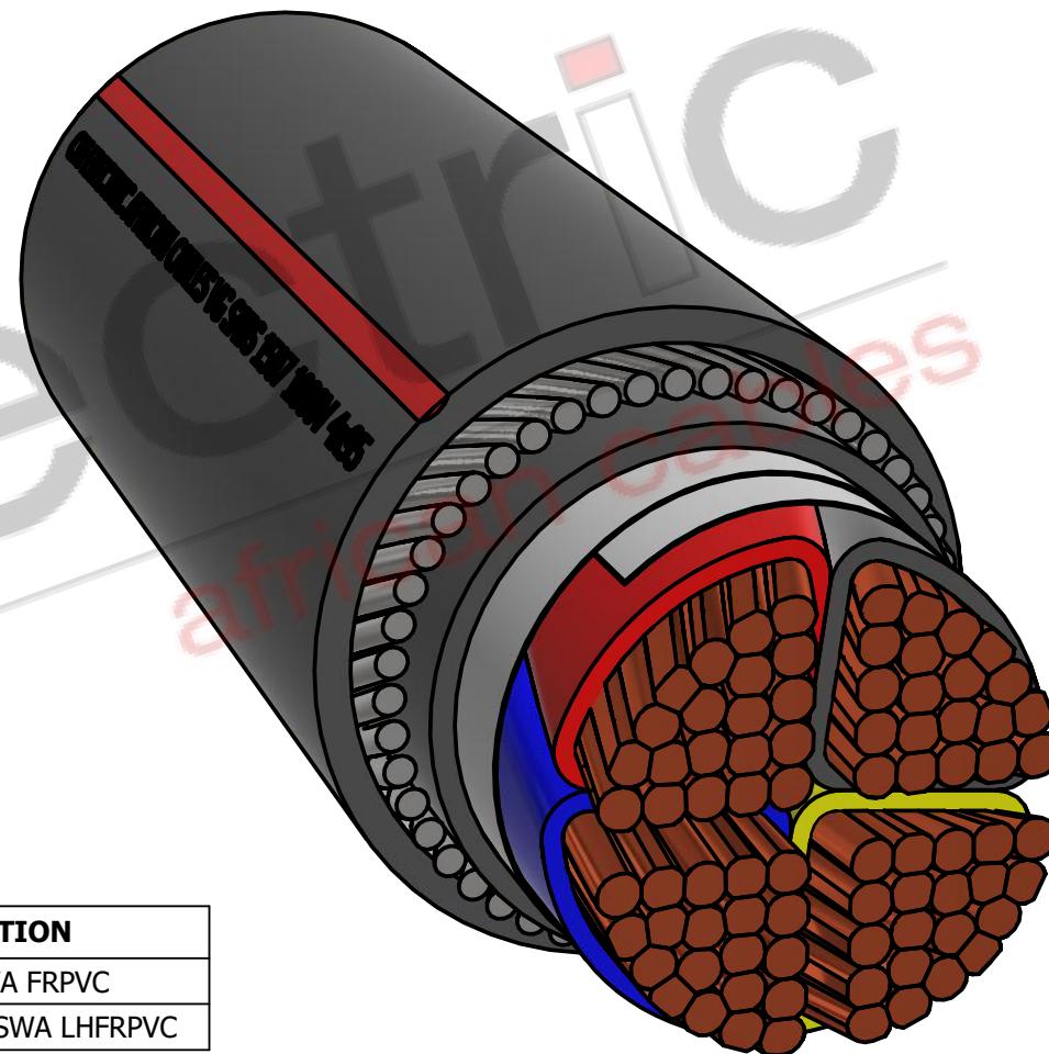
ISOMETRIC VIEW
