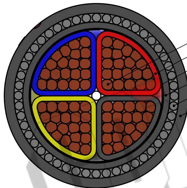
SECTIONAL VIEW
