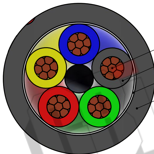
SECTIONAL VIEW
