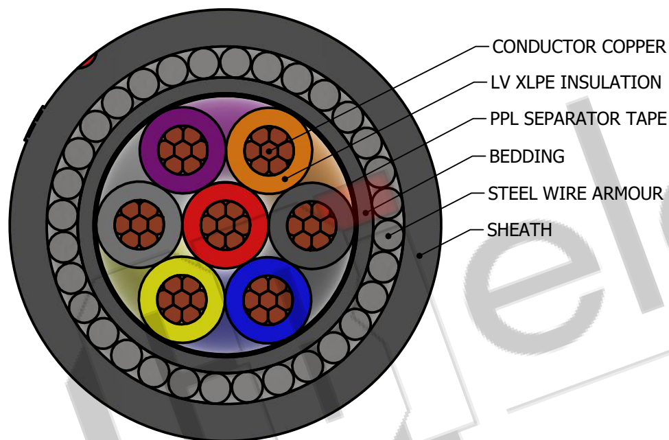
SECTIONAL VIEW
