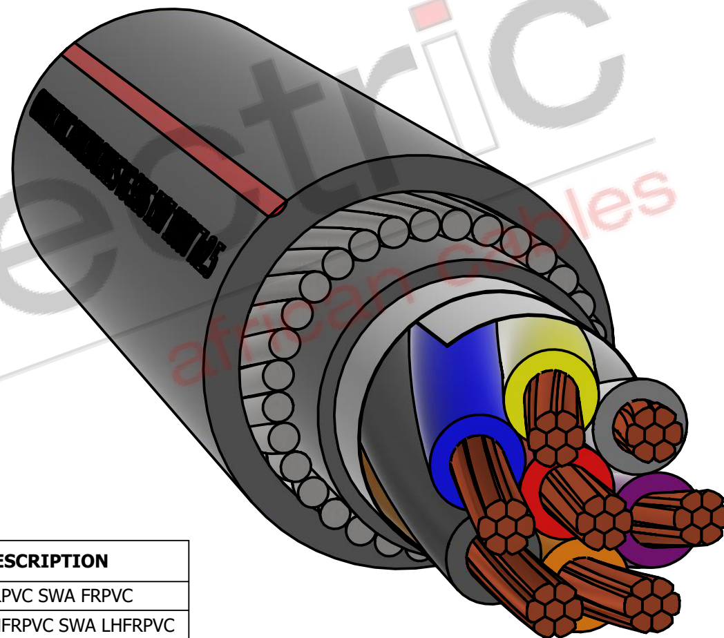
ISOMETRIC VIEW
