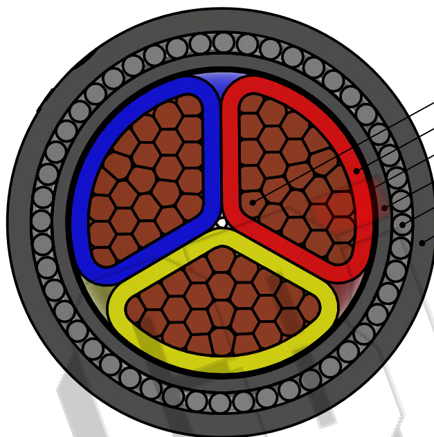
SECTIONAL VIEW
