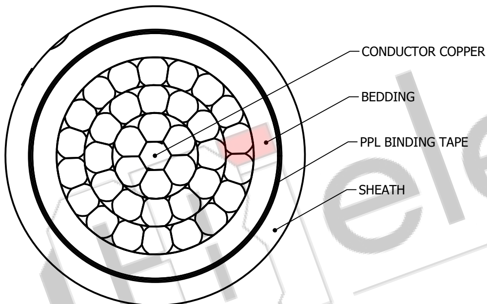
SECTIONAL VIEW
