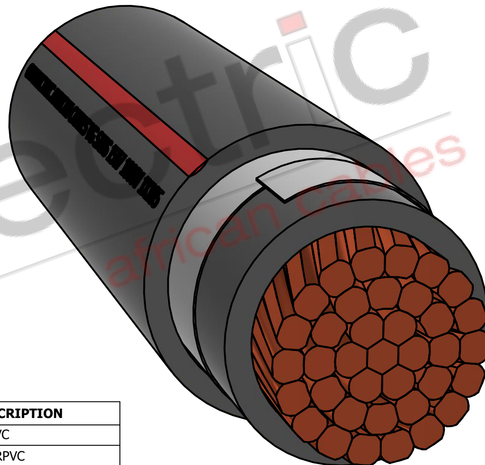
ISOMETRIC VIEW
