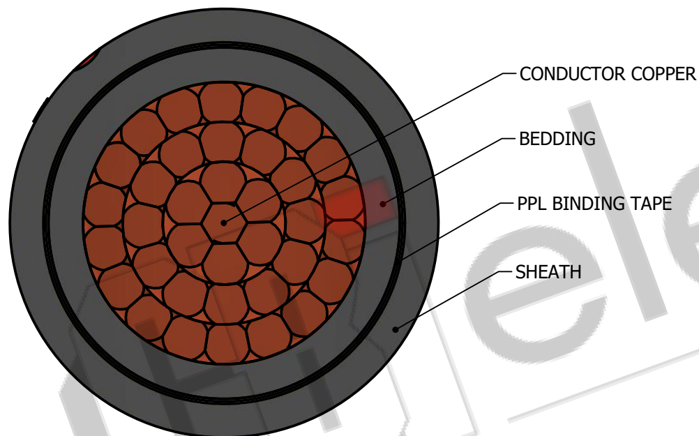
SECTIONAL VIEW
