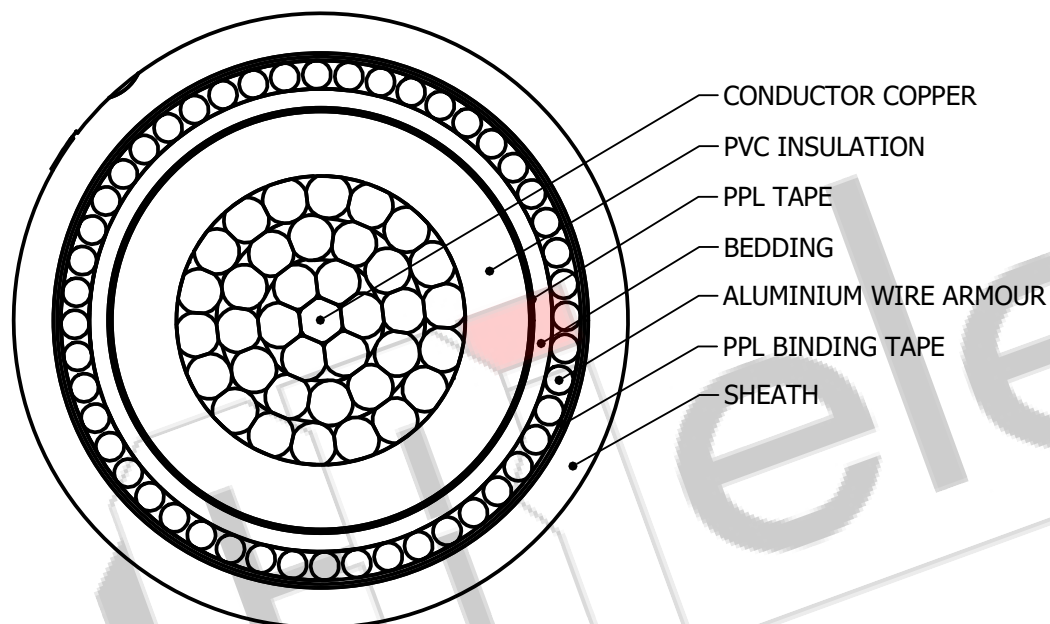
SECTIONAL VIEW
