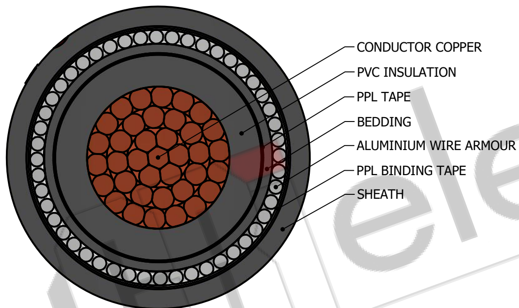
SECTIONAL VIEW
