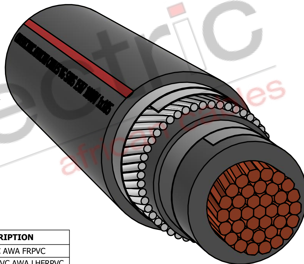
ISOMETRIC VIEW
