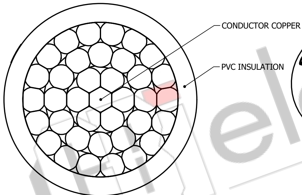
SECTIONAL VIEW
