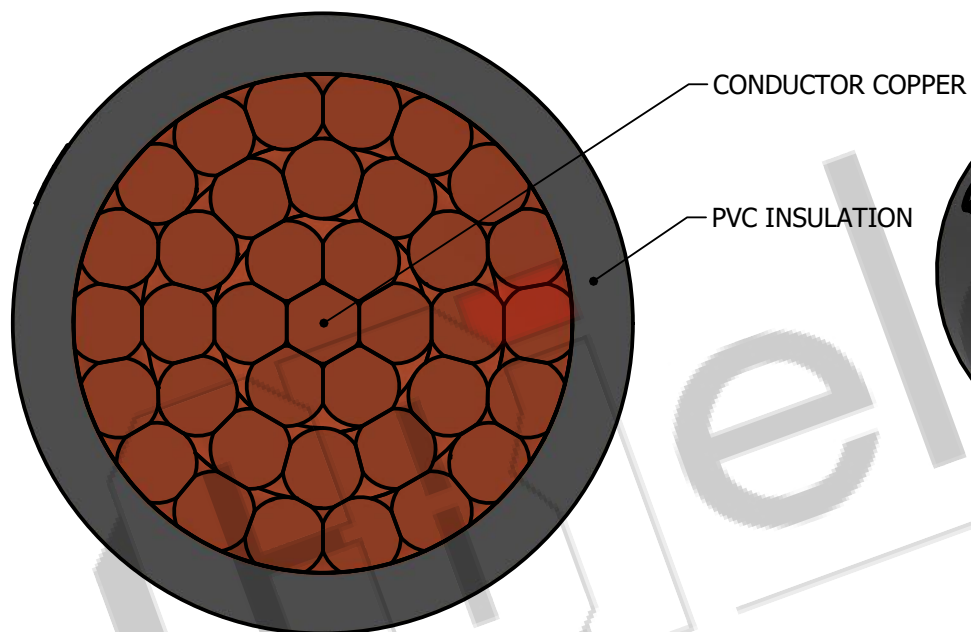
SECTIONAL VIEW
