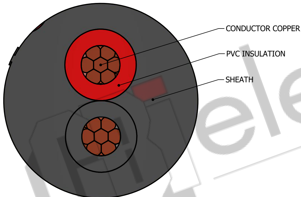
SECTIONAL VIEW
