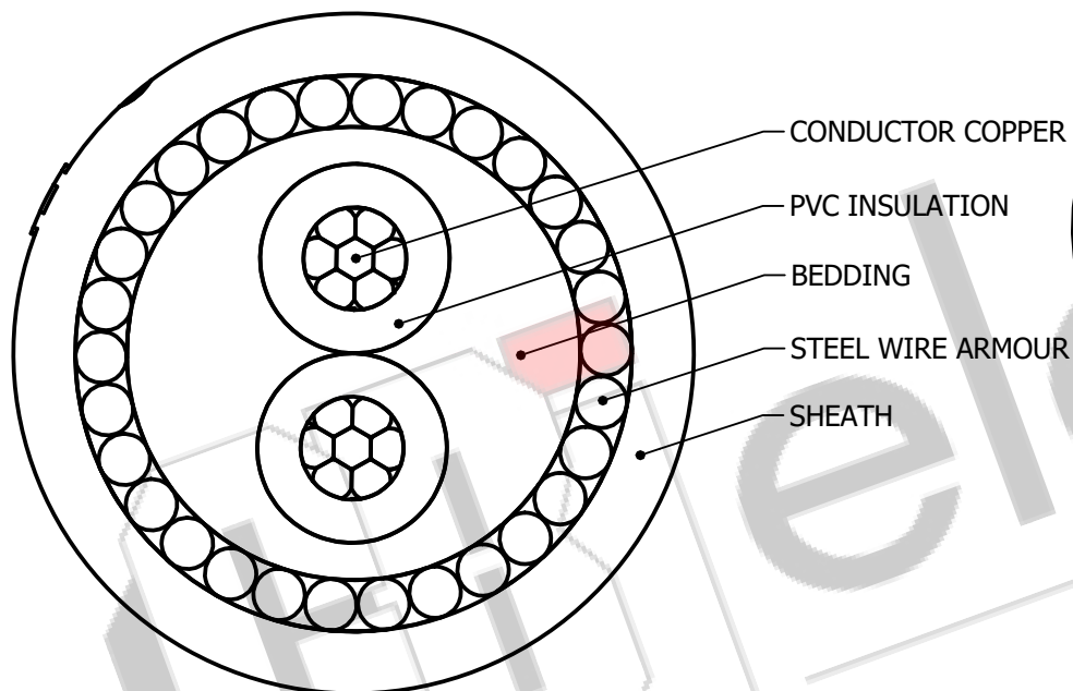
SECTIONAL VIEW
