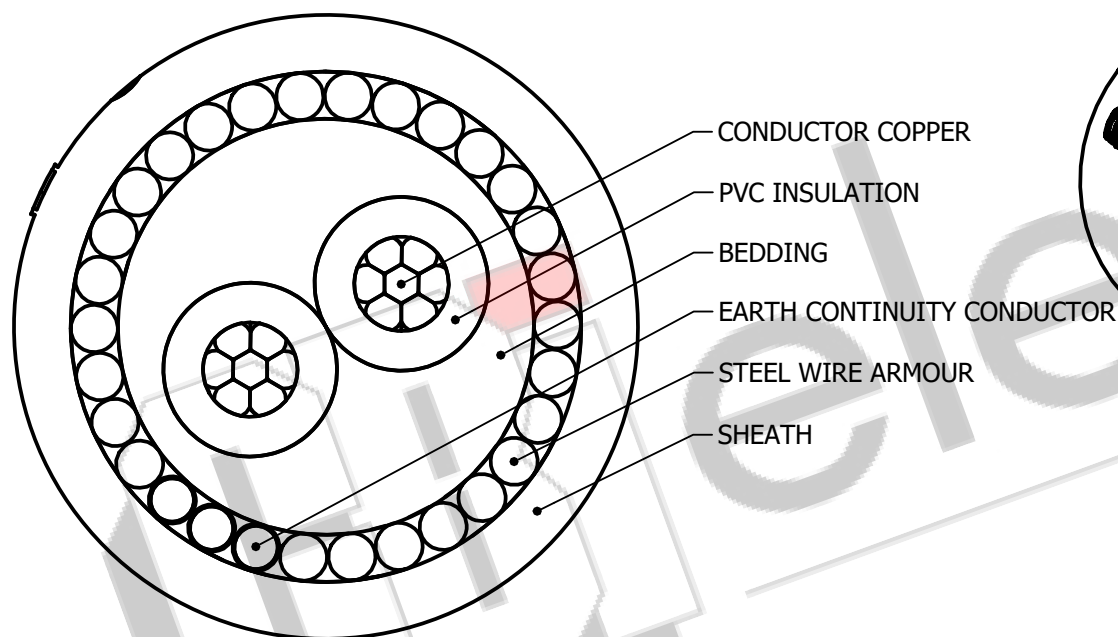
SECTIONAL VIEW
