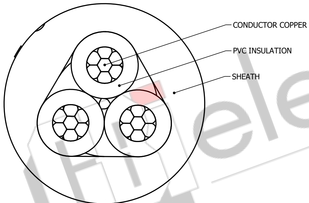
SECTIONAL VIEW
