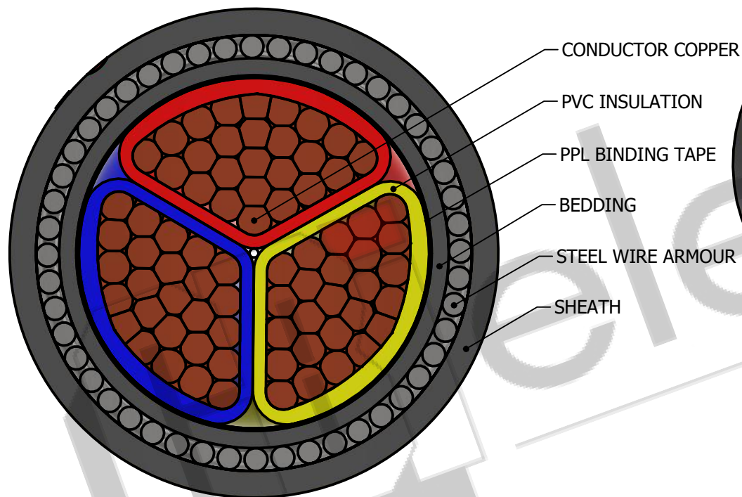
SECTIONAL VIEW
