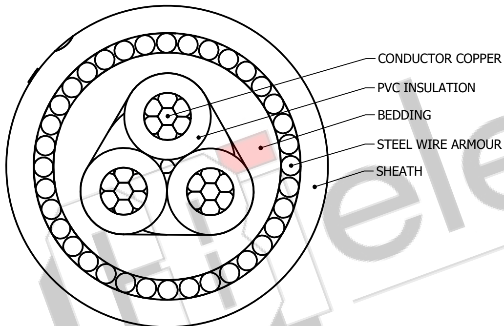
SECTIONAL VIEW
