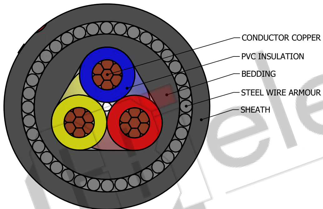
SECTIONAL VIEW
