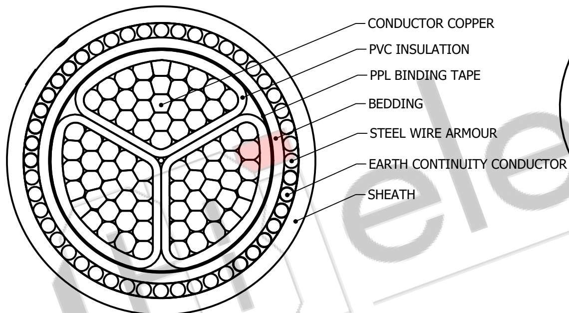
SECTIONAL VIEW
