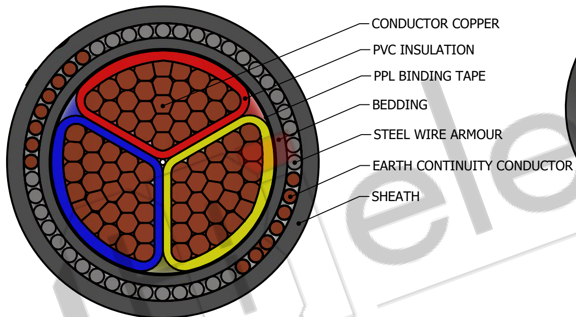
SECTIONAL VIEW
