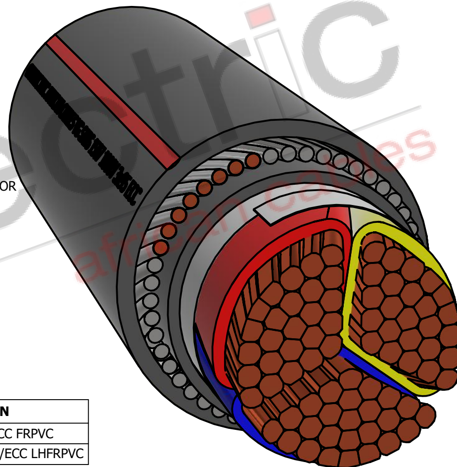
ISOMETRIC VIEW
