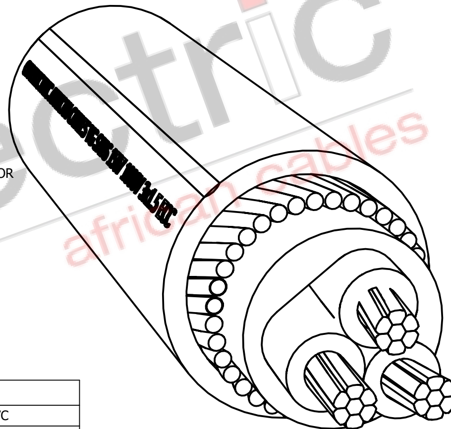
ISOMETRIC VIEW
