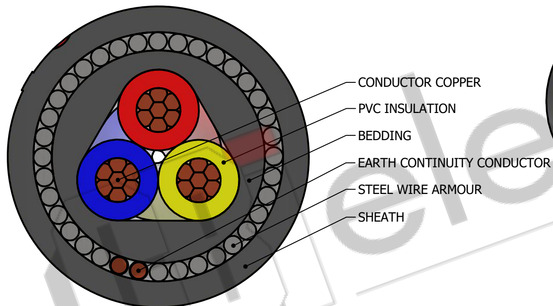
SECTIONAL VIEW
