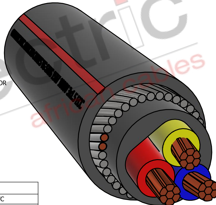
ISOMETRIC VIEW
