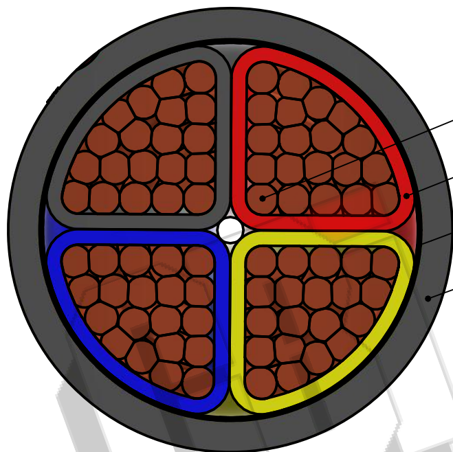
SECTIONAL VIEW
