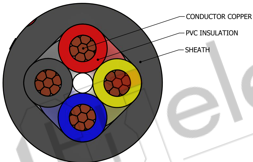
SECTIONAL VIEW
