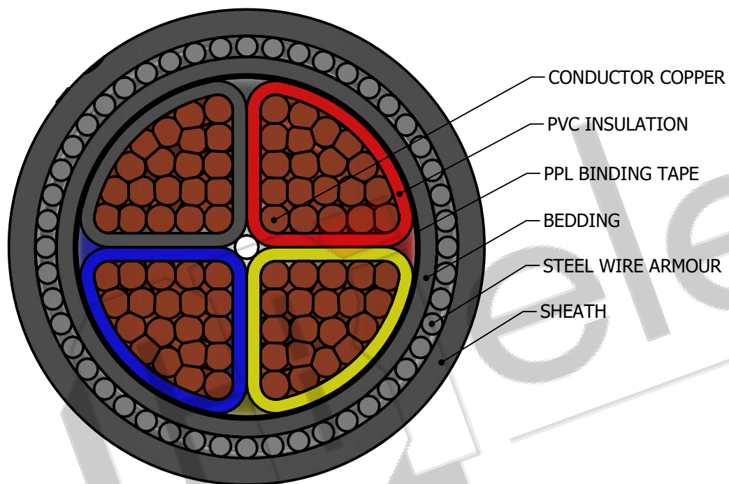
SECTIONAL VIEW
