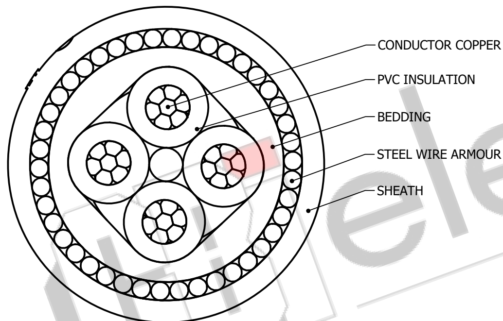
SECTIONAL VIEW
