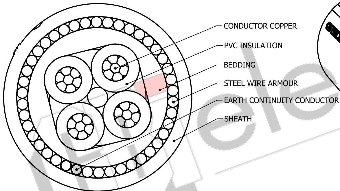
SECTIONAL VIEW
