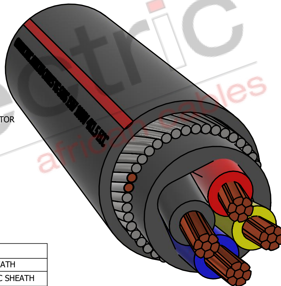
ISOMETRIC VIEW
