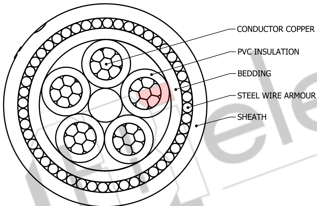
SECTIONAL VIEW
