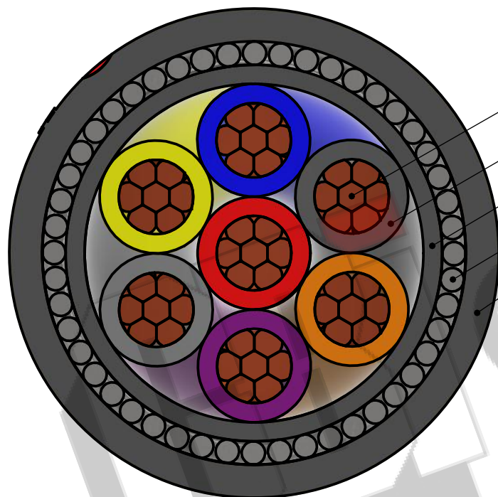
SECTIONAL VIEW
