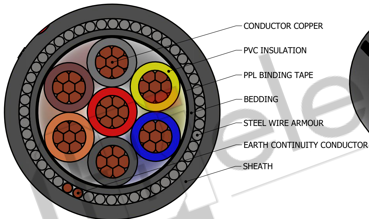
SECTIONAL VIEW
