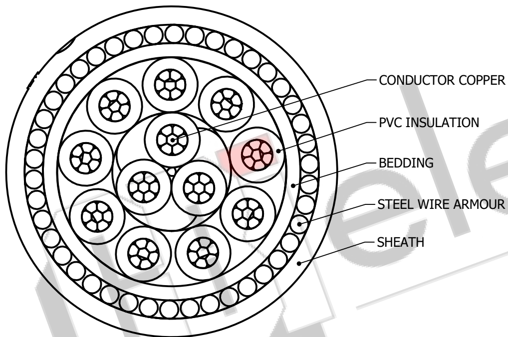
SECTIONAL VIEW
