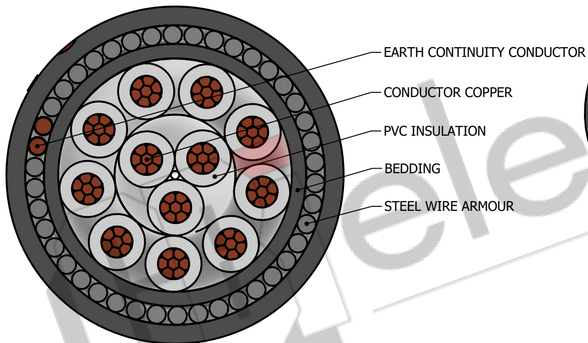
SECTIONAL VIEW
