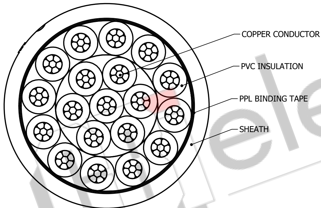
SECTIONAL VIEW
