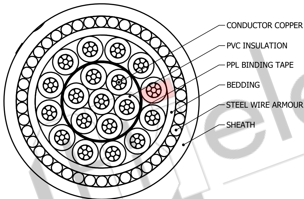
SECTIONAL VIEW
