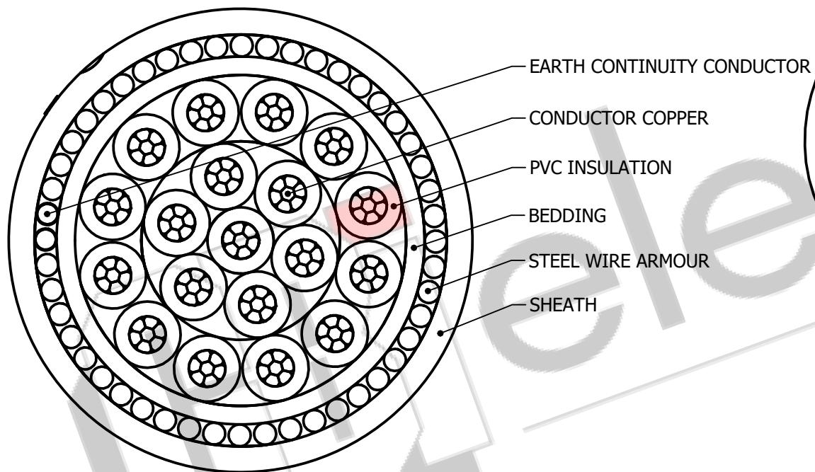
SECTIONAL VIEW
